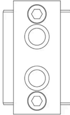
Alignment Fixture AT for T- and U-rails
