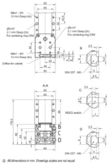
① All dimensions in mm. Drawings scales are not equal.
