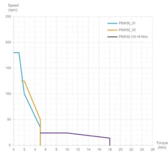
Performance Curve - Direct Drives PSW
